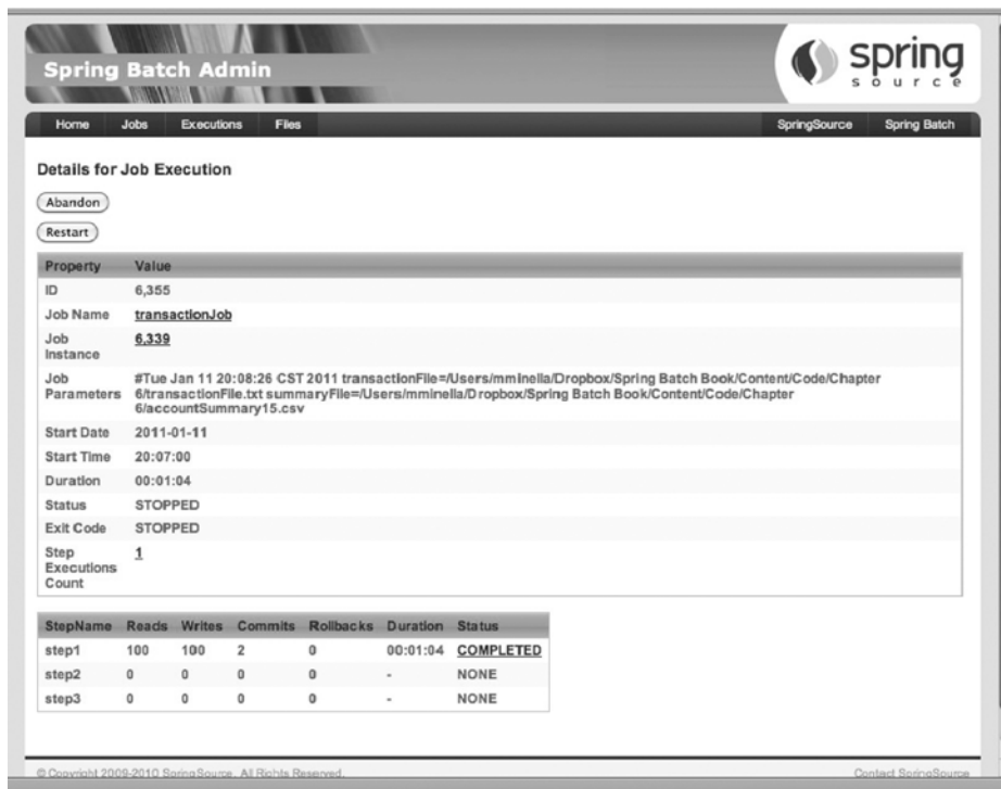
Figure 6-7. Results of the first run of transactionJob
